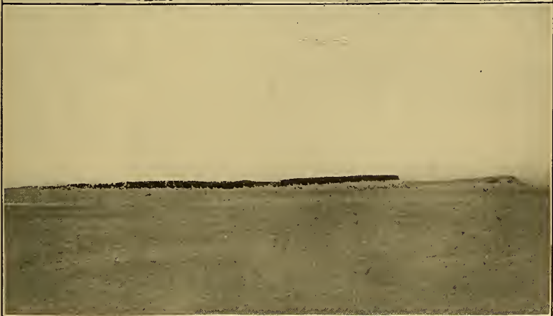
1. COLUMNAR BASALT UNDERLAID BY STRATIFIED LIMESTONE.
