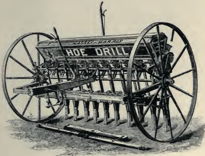
56. GRAIN DRILL.
