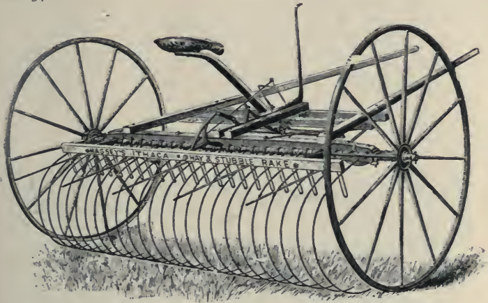
82. HORSE RAKE.
