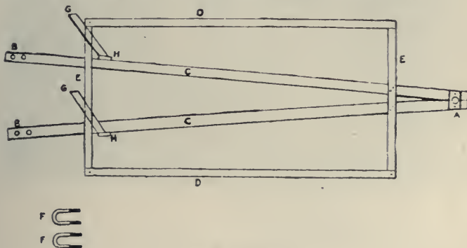
71. CORN PLATFORM.
