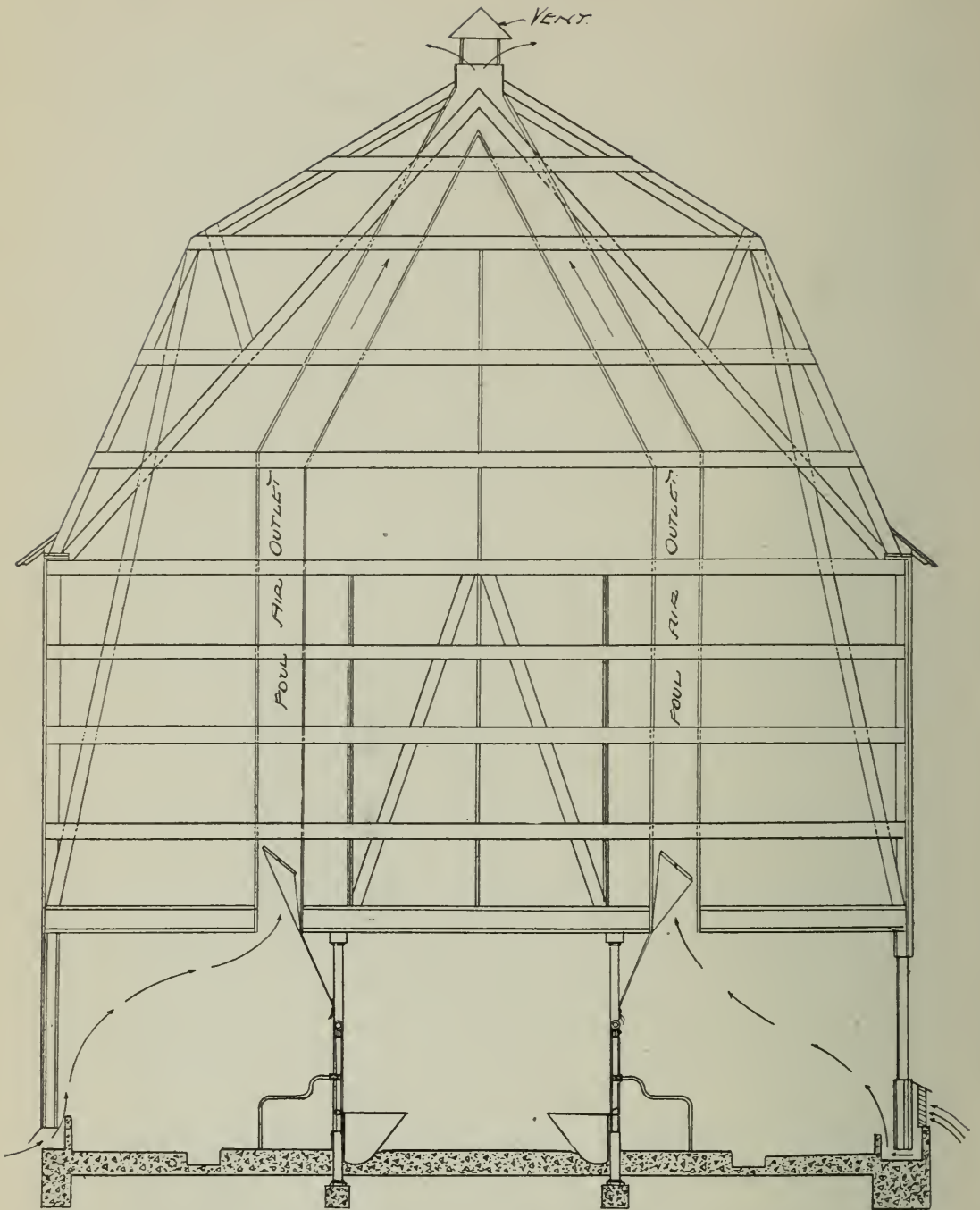
RUTHERFORD SYSTEM OF VENTILATION.
