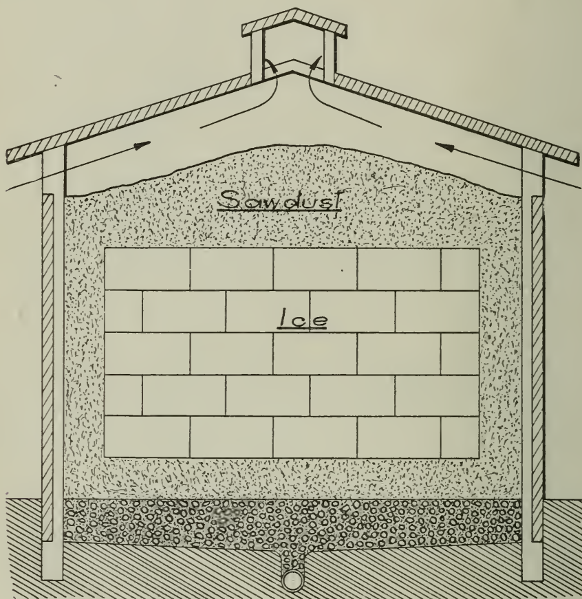
Fig. 4.—Cheap Ice-House.
