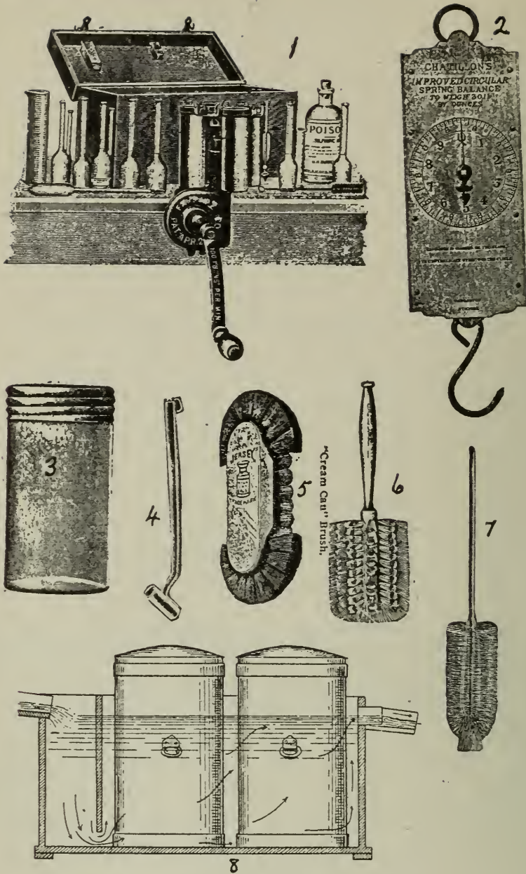
Figure 1—4-bottle Hand Babcock Test Outfit.
