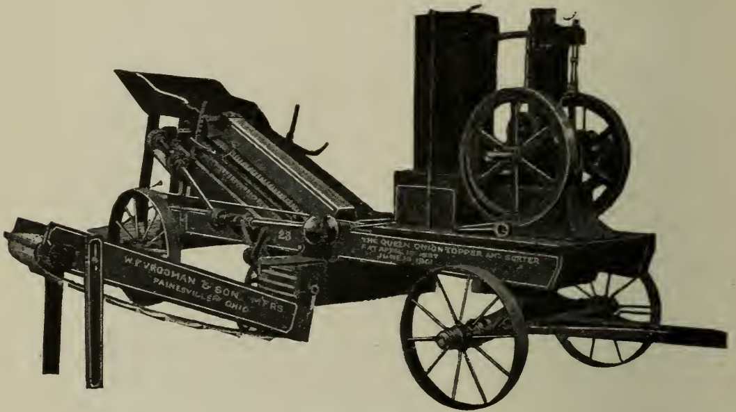
Onion Topper.
