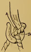
FIG. 27.—BLACKWALL HITCH.
