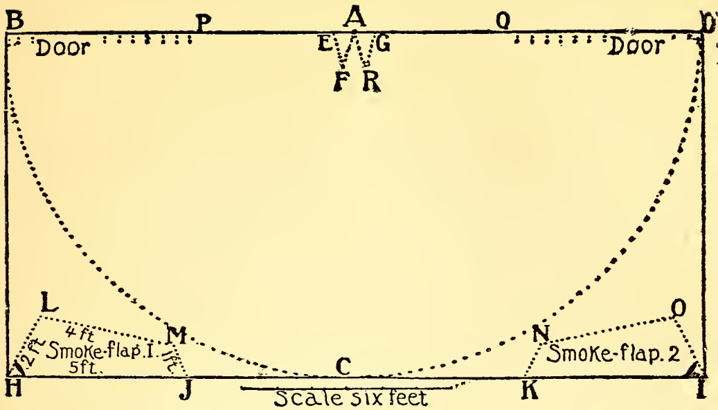
CUT I.—PATTERN FOR A SIMPLE 10-FOOT TEEPEE
