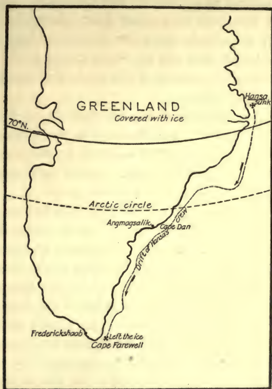
Southeastern Greenland.
