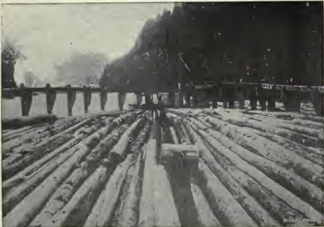
(2). Benson Raft under construction, showing upper part of cradle. Photo by Gifford and Prentiss, Portland, Oregon.
