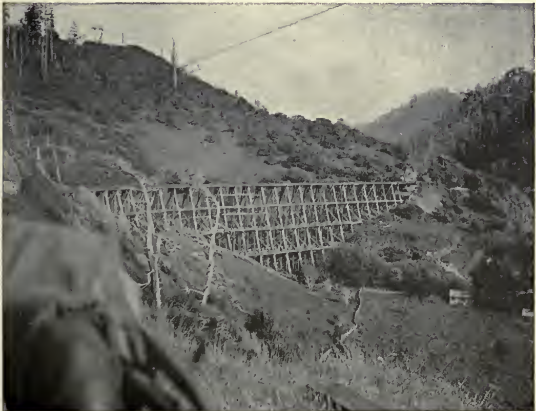
(2). Trestle 240 feet long and 150 feet high, 3 feet track.—Elk, California.
