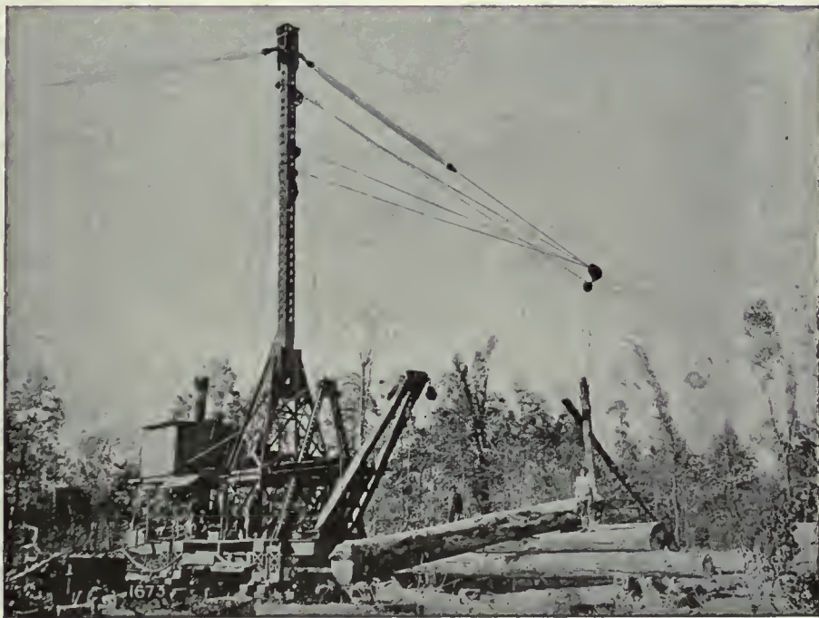
(2). Lidgerwood Overhead Skidder, lowering steel spar type, with swinging loading boom.
