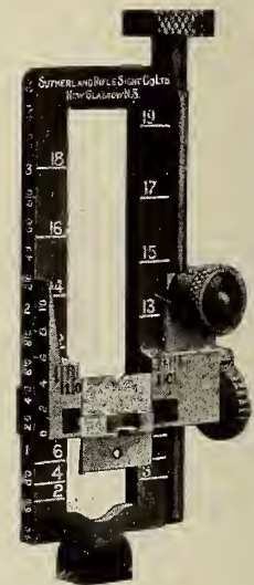
Sutherland Rifle Sight, Mark III.
