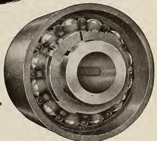
LOOSE PULLEY BEARING
