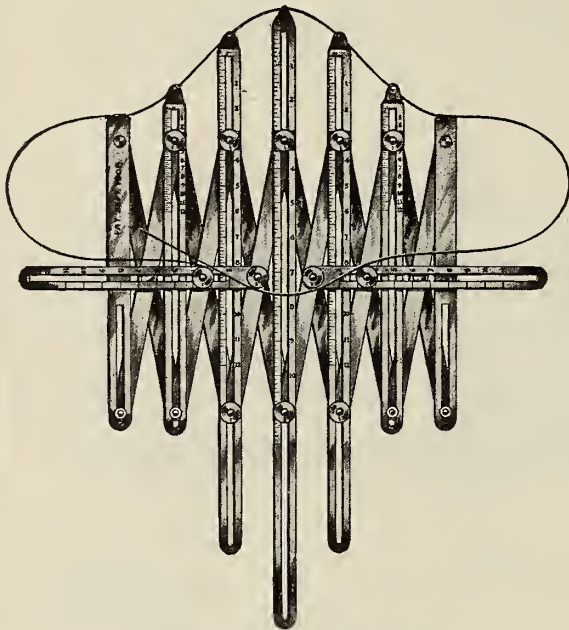
Universal Pipe Elbow Pattern
