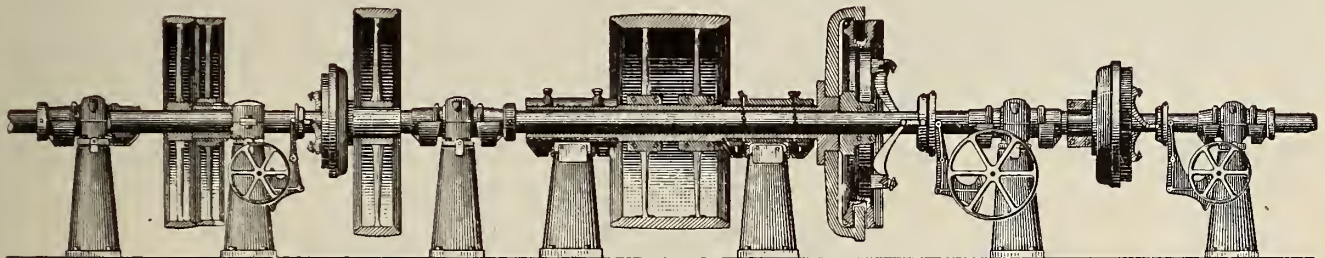
Dodge Jack Shaft Showing Friction Clutch and Quill Arrangement
