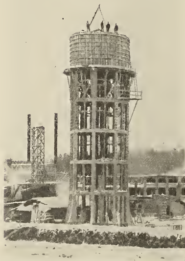
A Cement Water Tank—The First of the Kind Built in Canada. The Wood Products Co. Factory.
