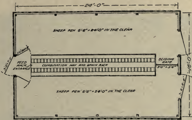
Floor plan of closed sheep-shed.
