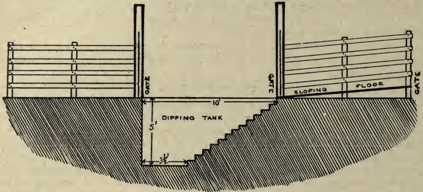
Illustration of a type of dipping-tank for a small flock.
