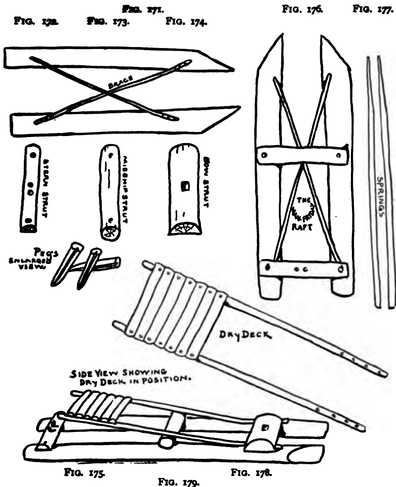
FIG. 171.—Logs in Place with Braces. FIGS. 172, 173, and 174.—Struts. FIG. 175.—Pegs. FIG. 176.—Raft with Middle and Stern Strut in Place. FIG. 177.—Springs for Dry Deck. FIG. 178.—Dry Deck. FIG. 179.—Dry Deck in Place.
