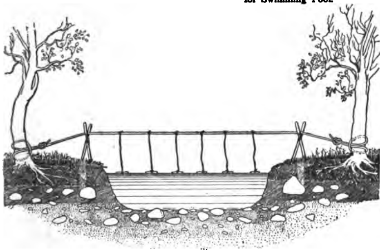
FIG. 252.—Diagram Showing the Suspension Bridge and Cross Section of Ground and Water.
