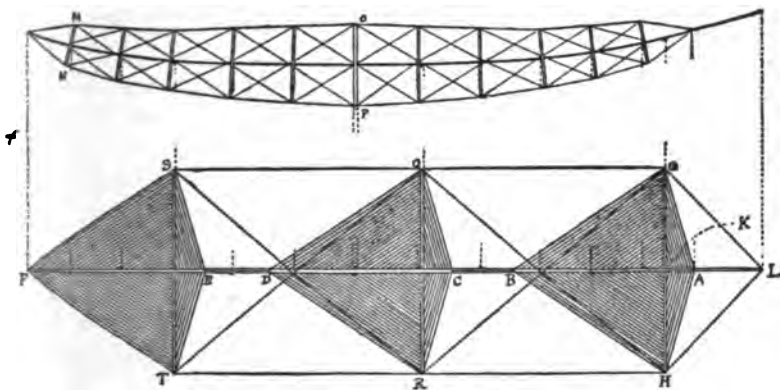
FIG. 38.—The Professional's Compound Kite.
