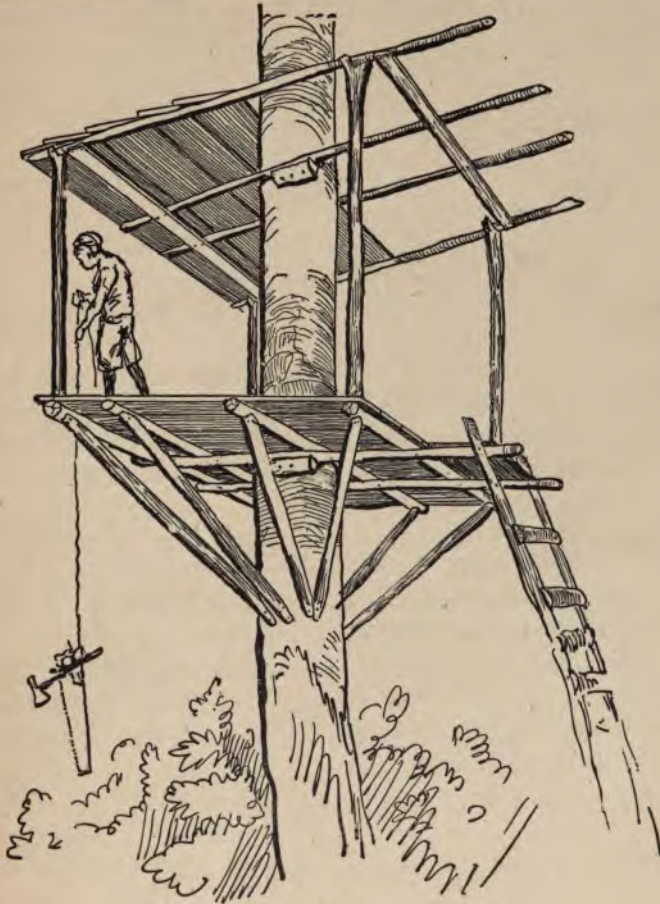
FIG. 6.—Frame of a One-Tree House.
