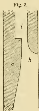
CORRECT CONSTRUCTION.
