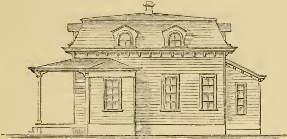
SIDE ELEVATION.
