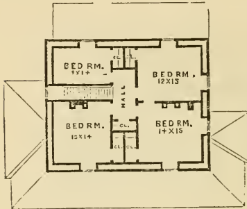
ATTIC. SECOND FLOOR PLAN.
