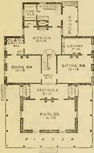
GROUND PLAN.
