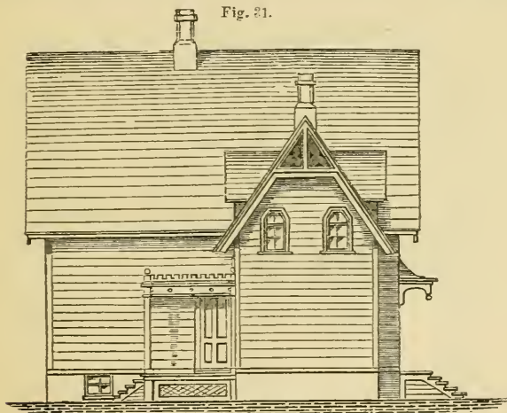
SIDE ELEVATION.
