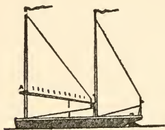
Fig. 164.—Sharpie with sprit and club leg-of-mutton sails.
