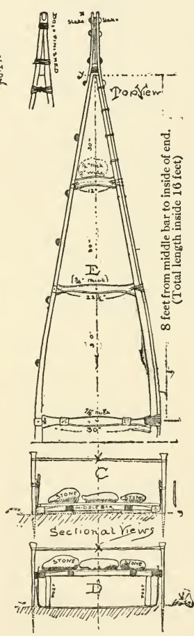
Fig. 85. Details of sticking and framework of canoe.
