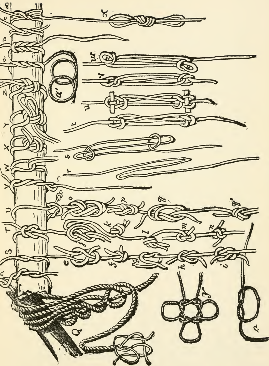
Pl. 187 1/2.—Timber-hitches, etc.
