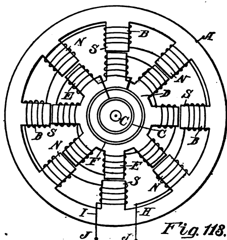
ALTERNATING CURRENT DYNAMO
