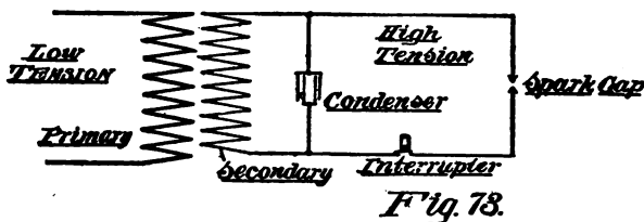
HIGH-TENSION CIRCUIT
