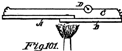
Fig. 101. THERMO-ELECTRIC COUPLE
