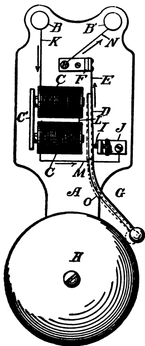
ELECTRIC BELL
