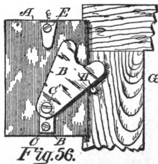
BURGLAR ALARM ATTACHMENT TO WINDOW
