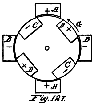
POSITIONS OF MAGNETS IN MOTOR
