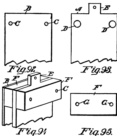
DETAILS OF PORTABLE PURIFIER
