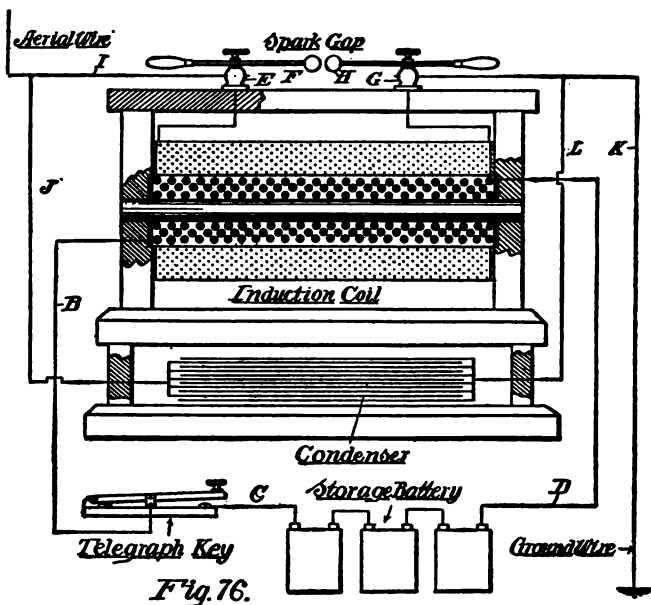
WIRELESS SENDING APPARATUS
