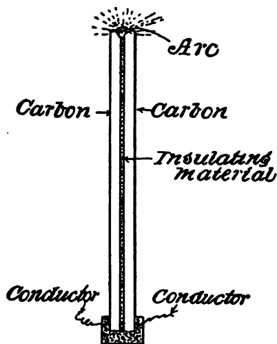
Fig. 116. Parallel Carbons.
