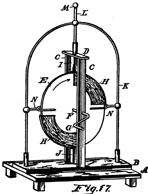
FRICTION-ELECTRICITY MACHINE
