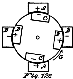
POSITIONS OF MAGNETS IN MOTOR
