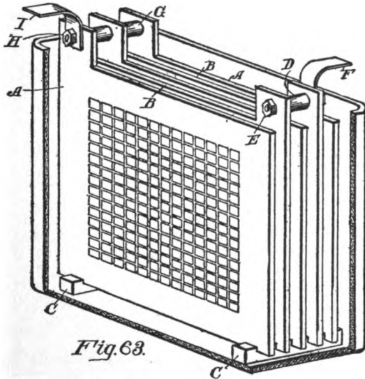
ASSEMBLAGE OF ACCUMULATOR PLATES
