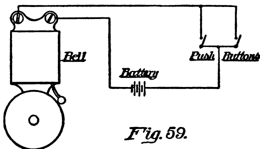
CIRCUITING FOR ELECTRIC BELL
