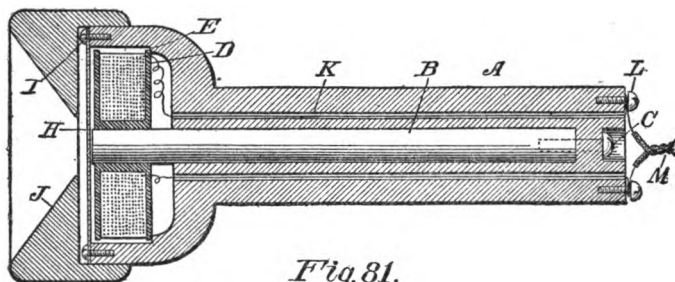
SECTION OF TELEPHONE RECEIVER
