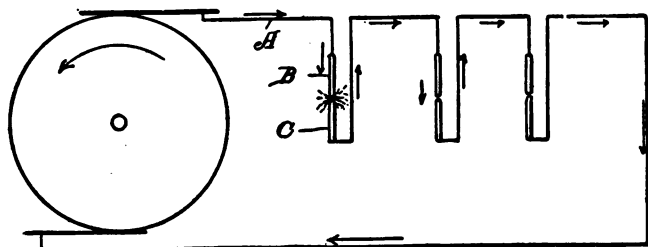
Fig. 117. Arc Lighting Circuit.
