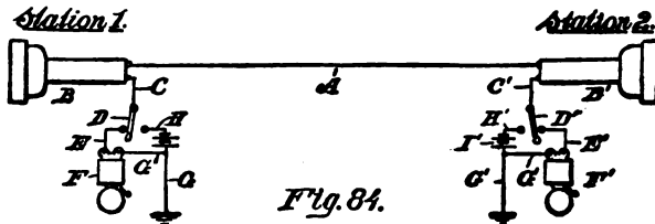
TELEPHONE STATIONS IN CIRCUIT
