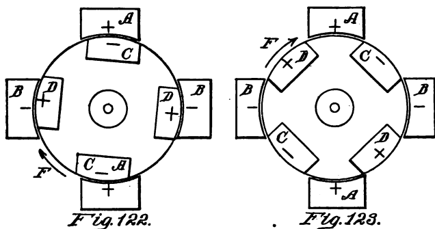
CYCLE ACTION IN DYNAMO
