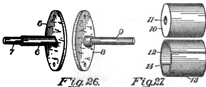
ARMATURE MOUNTINGS
