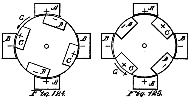
ACTION OF MAGNETS IN MOTOR
