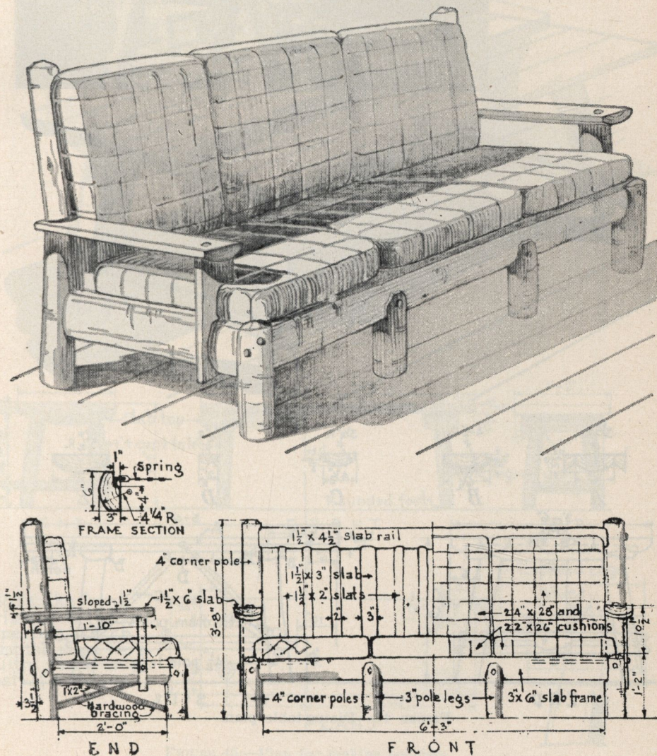
FIGURE 43.—Plan for making a living-room settee.
