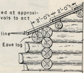
EAVE SECTIONS
