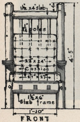
FIGURE 38.—Plan for making an armchair suitable for log residence.
