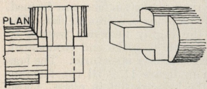
A VARIATION OF THE TENON
