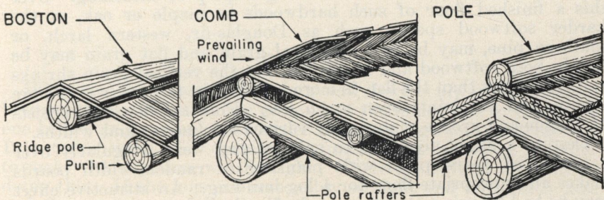
FIGURE 21.—Ridge treatments.
