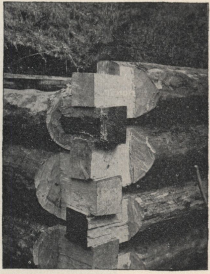
FIGURE 6.—Marking and framing the dovetail, or box, corner.
