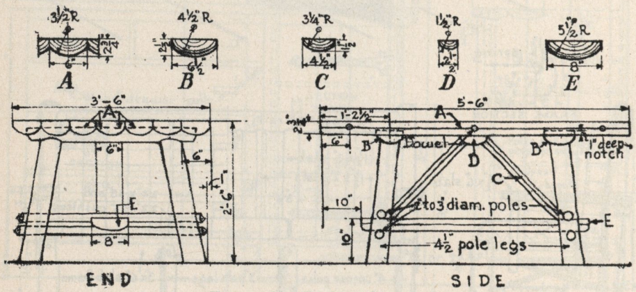
FIGURE 44.—Dining-table plan.
