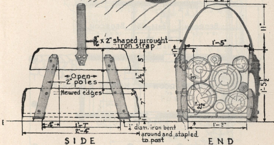
FIGURE 47.—Plan for a fireplace wood hod.
