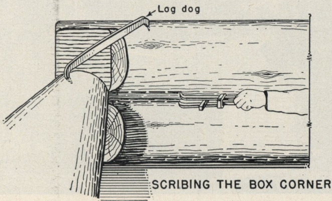
NORWEGIAN LOG SCRIBE
