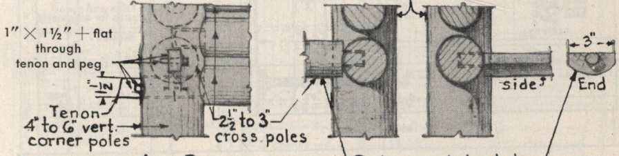
FIGURE 41.—Plan for building a double-deck bunk.
