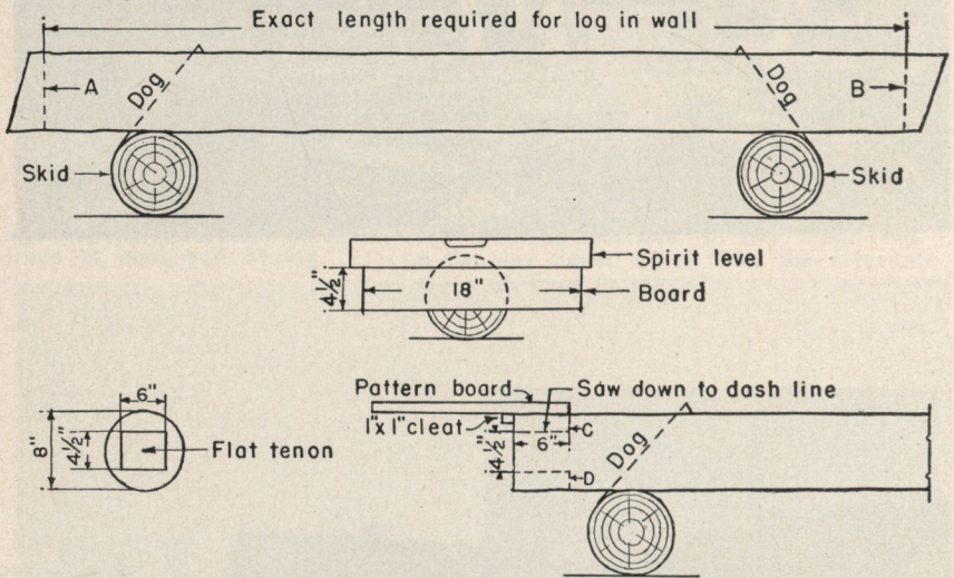
FIGURE 8.—Framing the flat, or plain, tenon corner.
