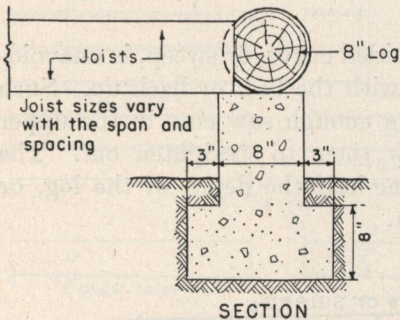
FRAMING SAWED FLOOR JOISTS
