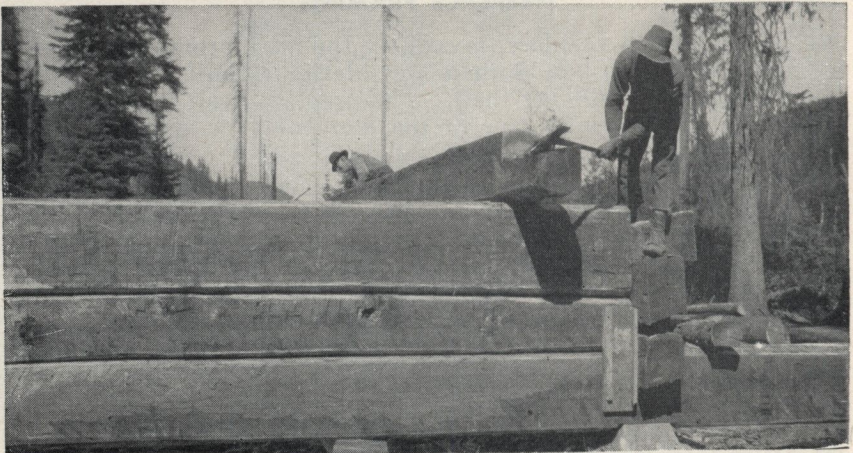
FIGURE 29.—Framing hewed timbers.
