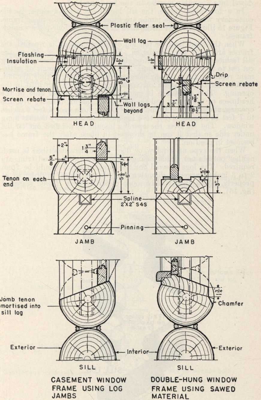
FIGURE 15.—Window frames.
