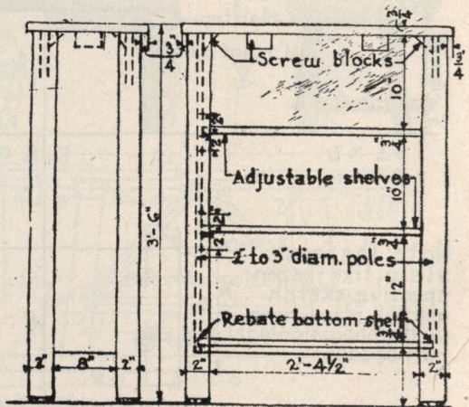
END FRONT
