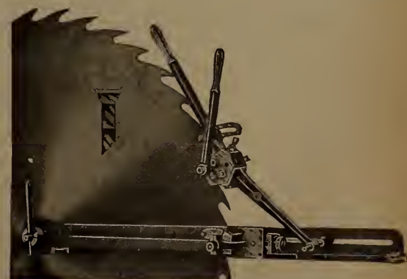
Hanchett Circular Saw Swage
