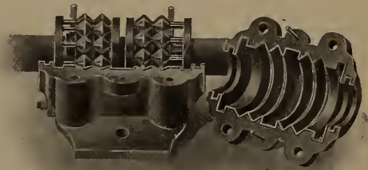
The Pillow Block Type of Bearing Showing Rollers in Double Series.
