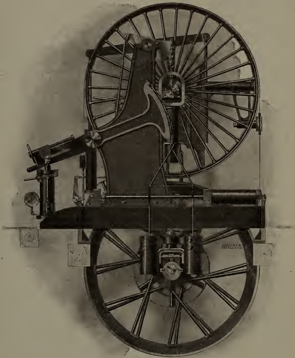
STEAM TENSION BAND MILL MANUFACTURED BY WM. HAMILTON MANUFACTURING CO.
