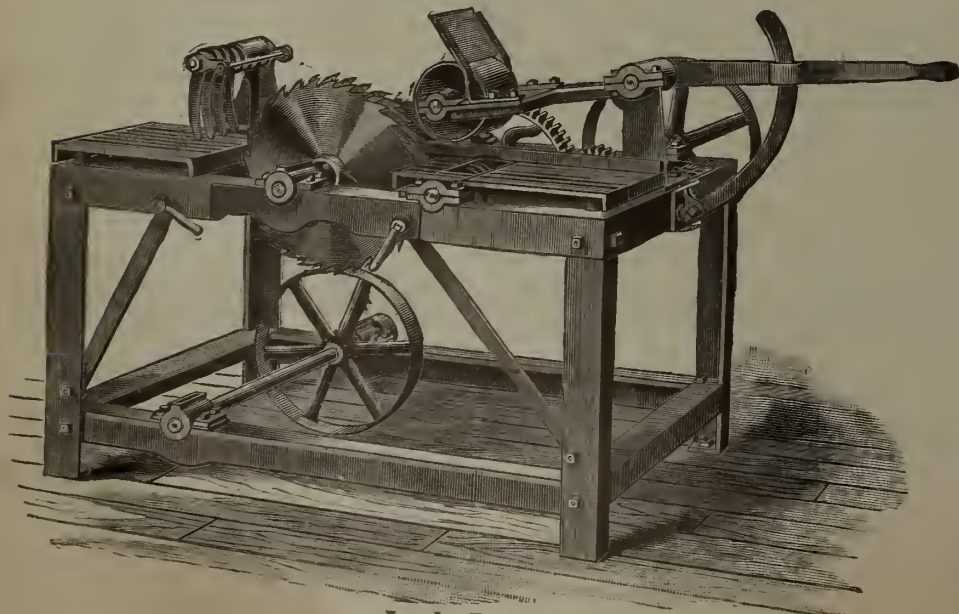
Lath Bolter
