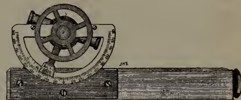
FIG. 6.—COMBINED SURVEYOR'S HAND LEVEL AND CLINOMETER.
